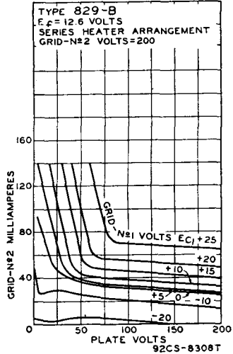
TYPICAL CHARACTERISTICS EACH UNIT
