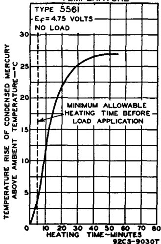
RATE OF RISE OF CONDENSED-MERCURY TEMPERATURE
