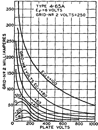
AVERAGE PLATE CHARACTERISTICS
